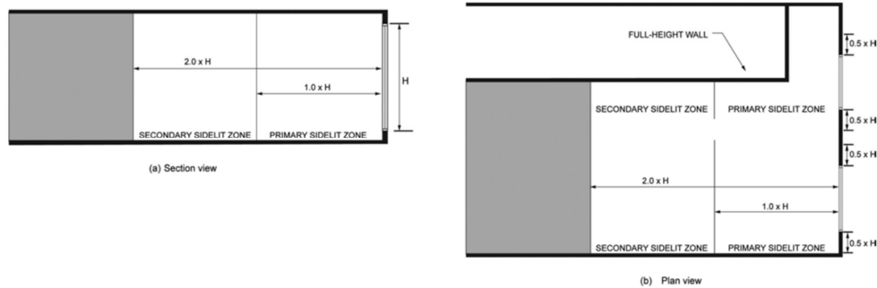
FIGURE C405.2.4.2(1) PRIMARY AND SECONDARY SIDELIT DAYLIGHT ZONES
