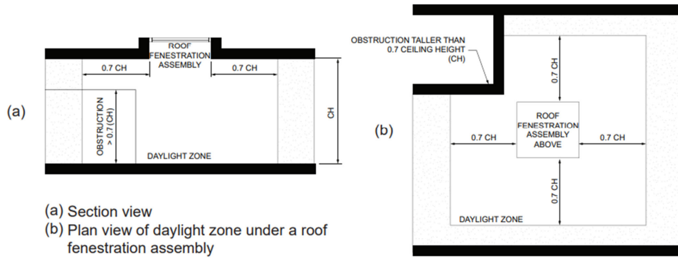
FIGURE C405.2.4.3(4)
