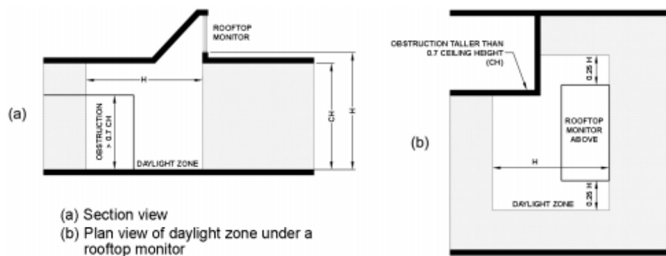
FIGURE C405.2.4.2(3) DAYLIGHT ZONE UNDER A SLOPED ROOFTOP MONITOR
