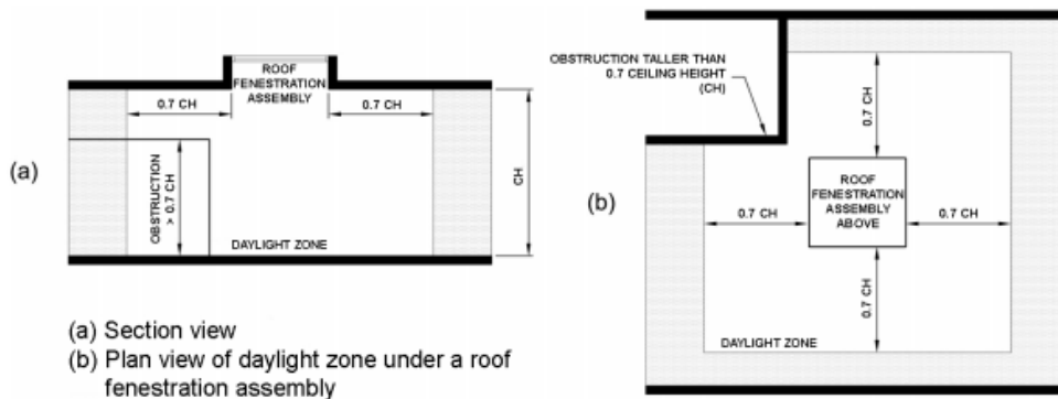
FIGURE C405.2.4.2(2) DAYLIGHT ZONE UNDER A ROOFTOP MONITOR
