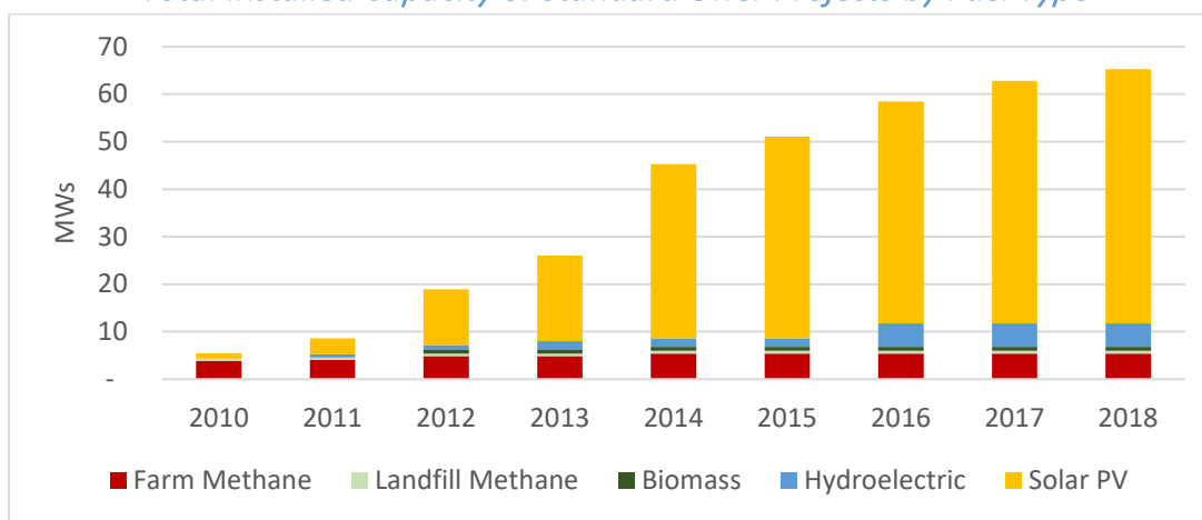
Figure 4: Capacity and Energy Provided by Standard Offer Projects by Fuel Type
