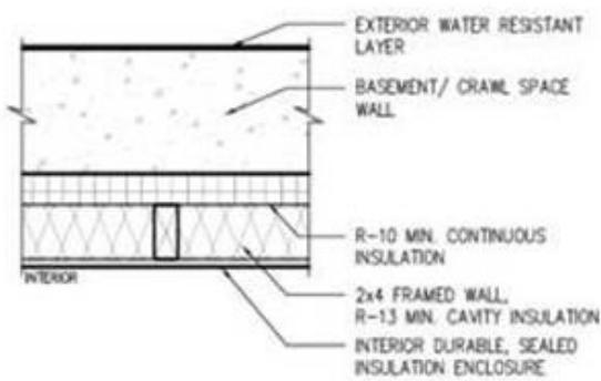
INTERIOR CAVITY + CONTINUOUS INSULATION
