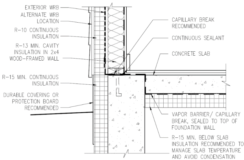
Figure 2.14 – Exterior foundation and sub-slab insulation with 2x4 above grade wall (R-13+10ci shown)
