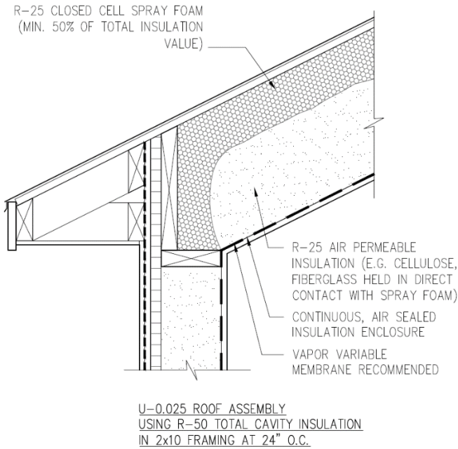
Figure 2.28 – “Flash and batt” hybrid cavity insulation
