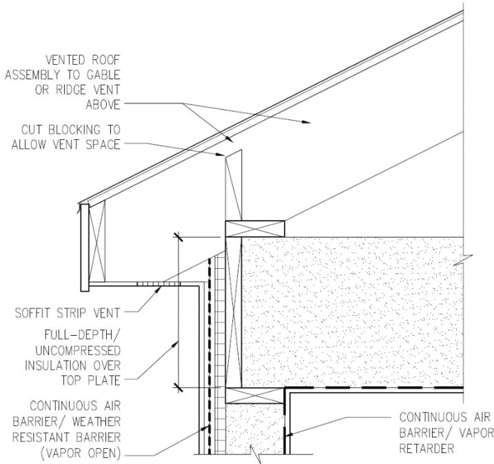
Figure 2.24 - Raised rafter
