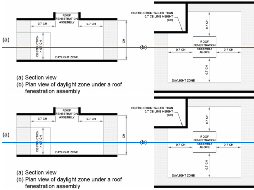
FIGURE C405.2.34.3(4) TOPLIT DAYLIGHT ZONE
